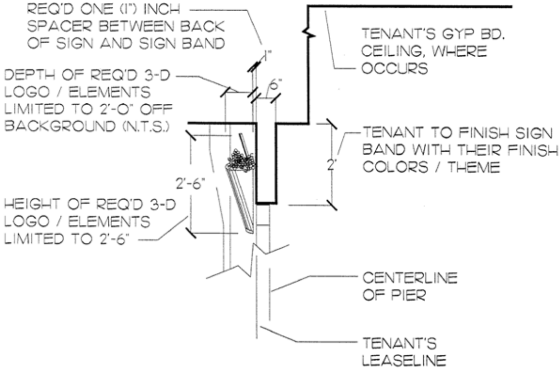
SECTION THROUGH TENANT'S SIGN BAND WITH NEUTRAL PIER BEYOND
